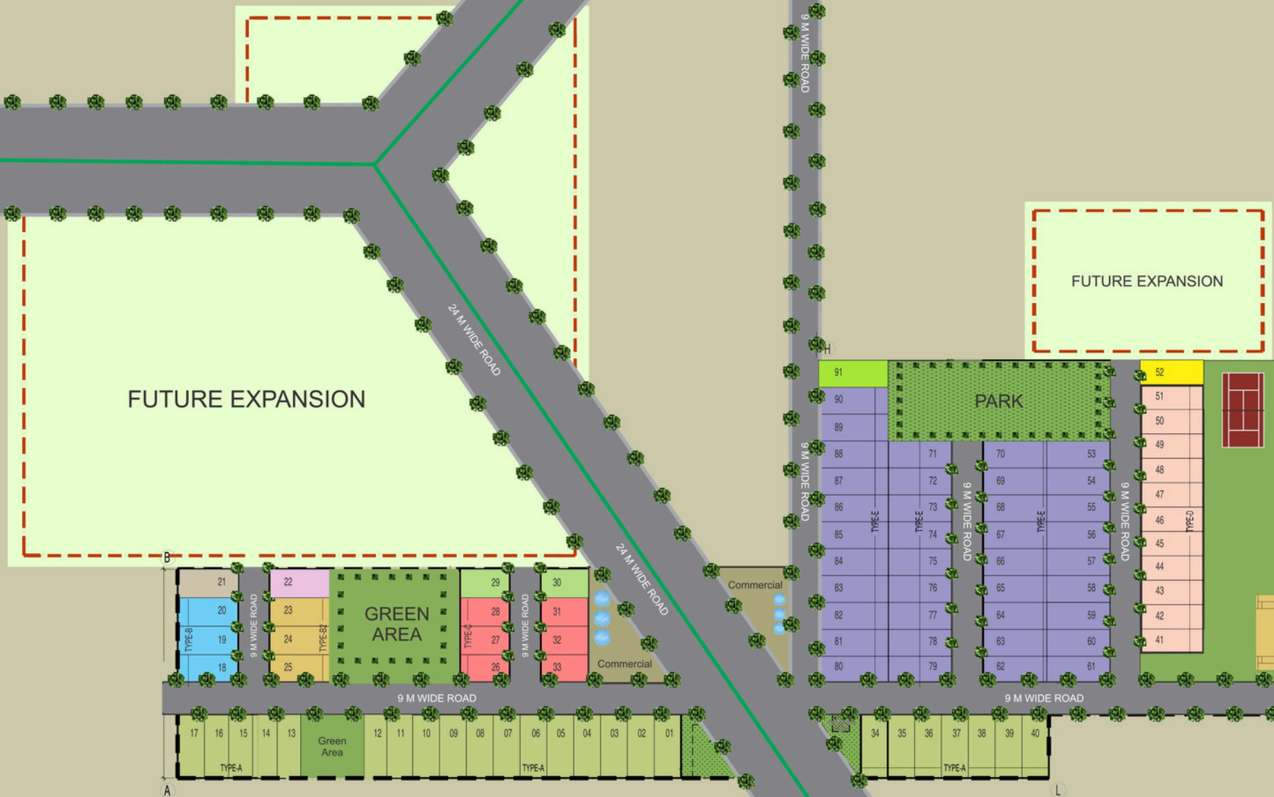
SITE LAYOUT
